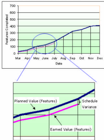
Figure 7. Burn-up chart & schedule variance.
