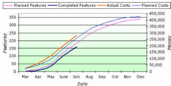
Figure 10. Burn-up chart with trimmed scope.
