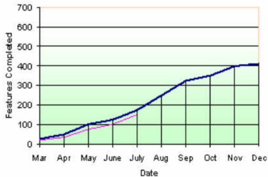
Figure 4. Sample burn-up chart.
