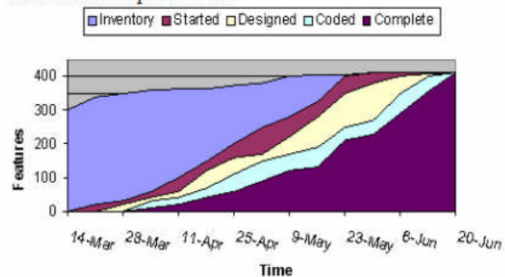
Figure 6. Sample cumulative flow diagram.
