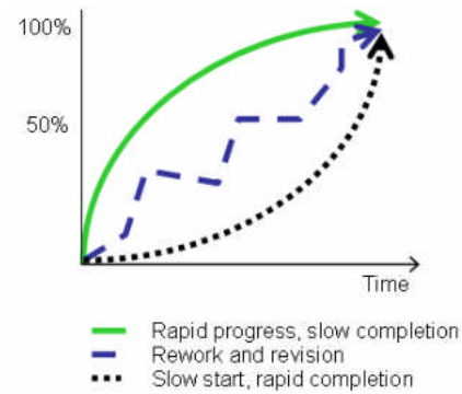
Figure 3. Agile software project progress.
