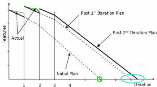
Figure 8. Burn-down chart reflecting scope and estimate changes.
